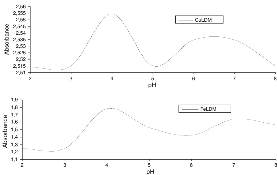
Fig. 3 The effect of pH on the complexes
